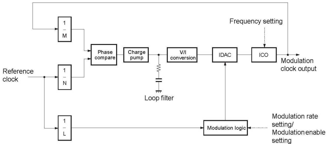
WAYCOI7368AG08CR PLL block
