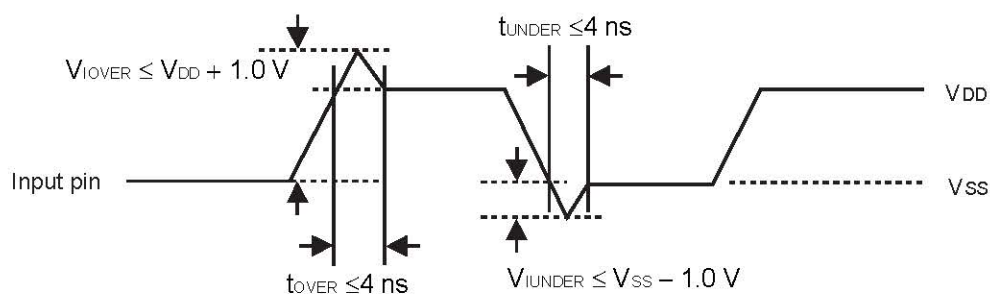
Overshoot/Undershoot
