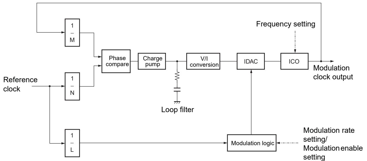
EMC73661108F PLL block
